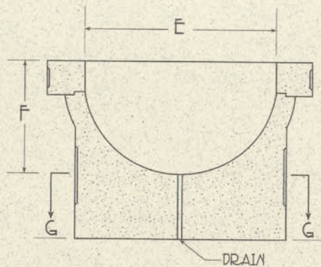
CUTAWAY
